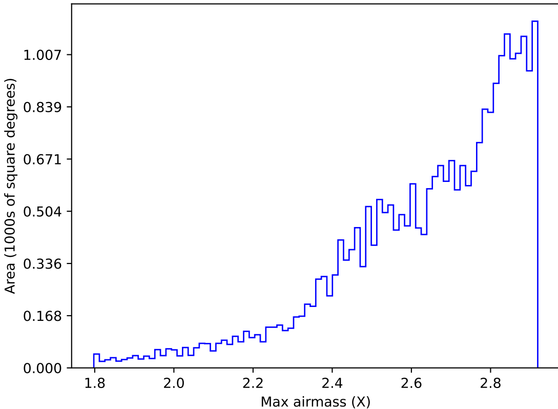
baseline_v3.2_10yrs All sky all bands: Max airmass
