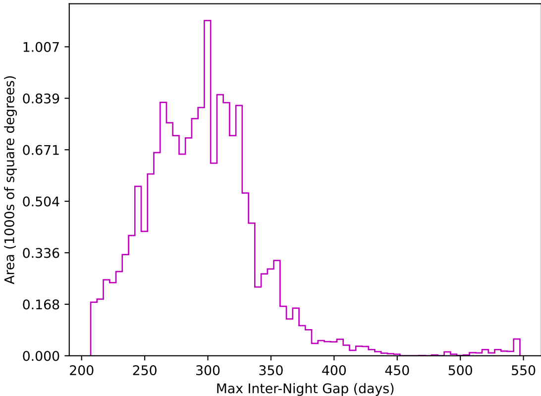
baseline_v3.2_10yrs WFD z band: Max Inter-Night Gap
