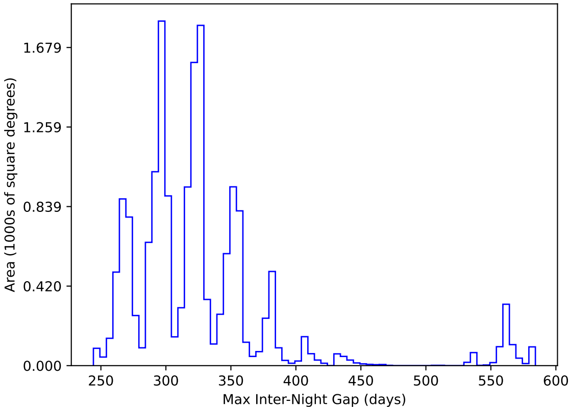
baseline_v3.2_10yrs WFD y band: Max Inter-Night Gap
