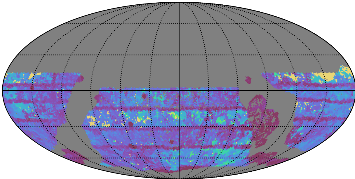
baseline_v3.2_10yrs WFD r band: Max Inter-Night Gap
