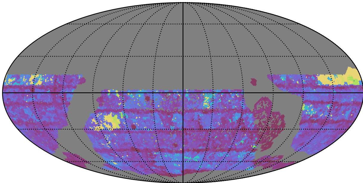
baseline_v3.2_10yrs WFD i band: Max Inter-Night Gap
