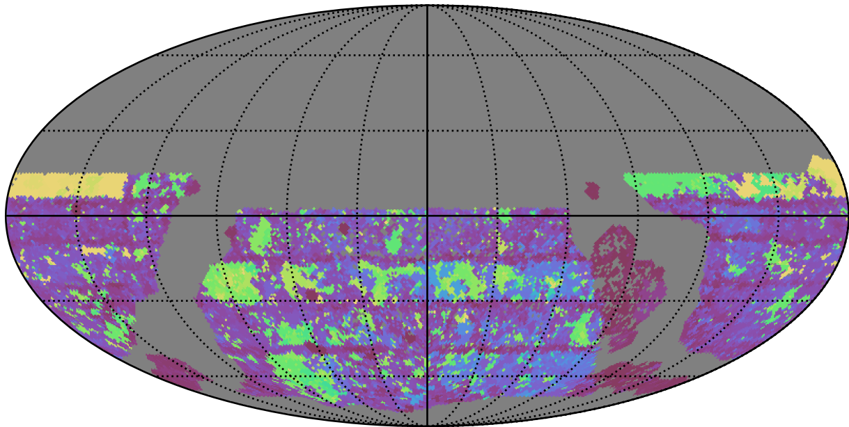
baseline_v3.2_10yrs WFD g band: Max Inter-Night Gap
