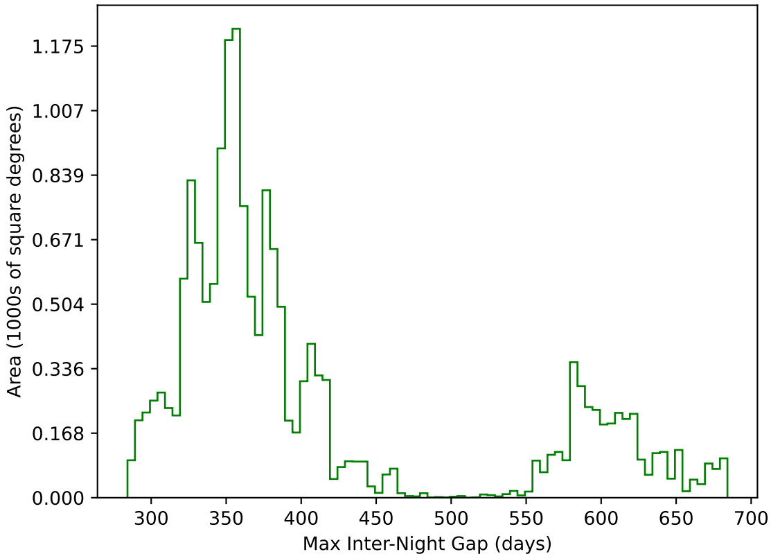
baseline_v3.2_10yrs WFD g band: Max Inter-Night Gap
