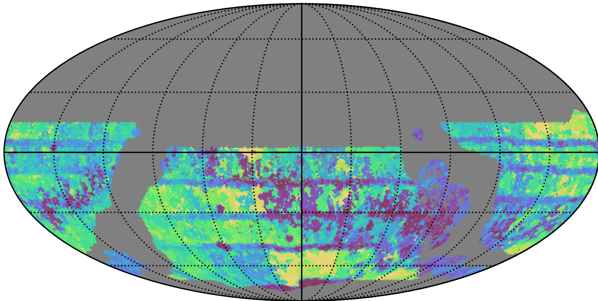
baseline_v3.2_10yrs WFD all bands: Max Inter-Night Gap
