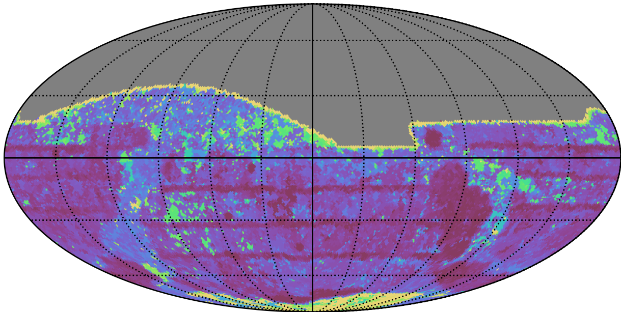
baseline_v3.2_10yrs All sky z band: Max Inter-Night Gap
