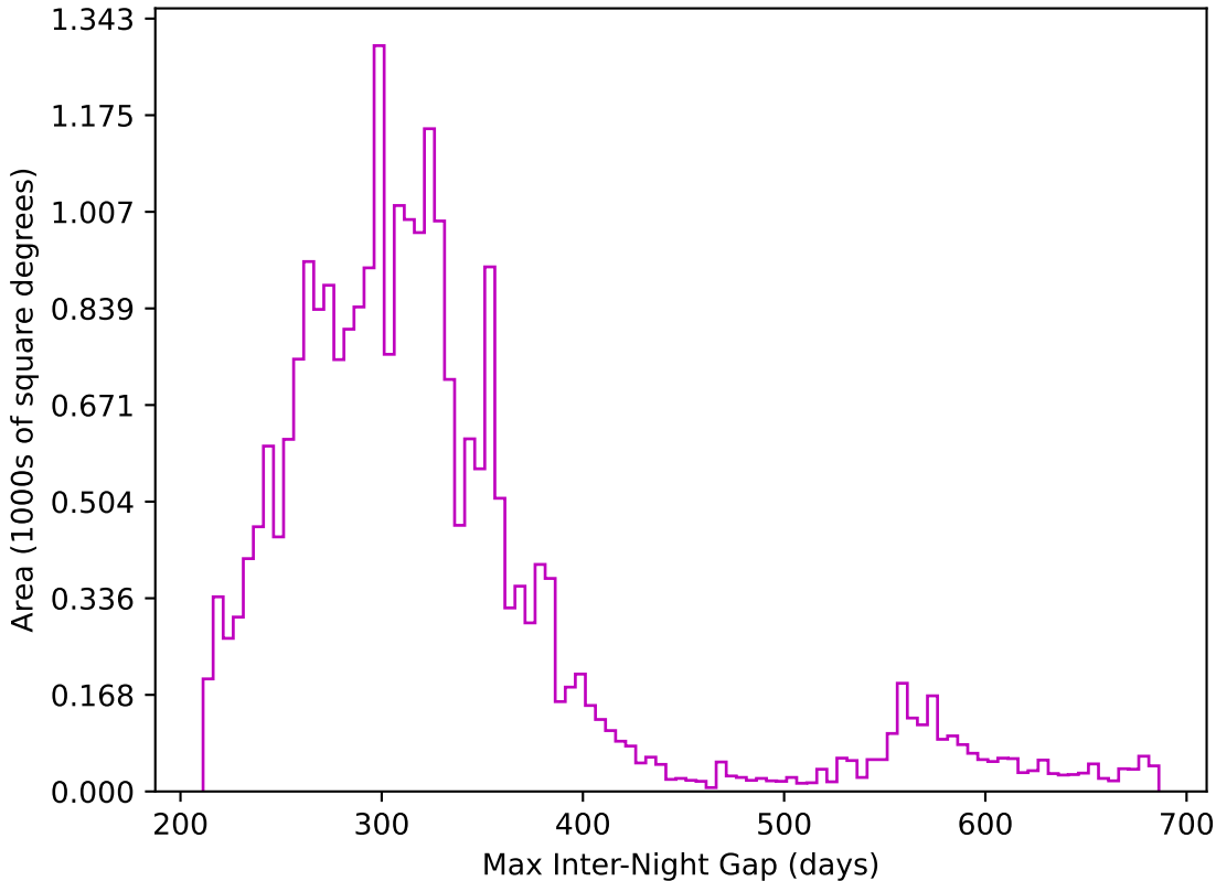
baseline_v3.2_10yrs All sky z band: Max Inter-Night Gap
