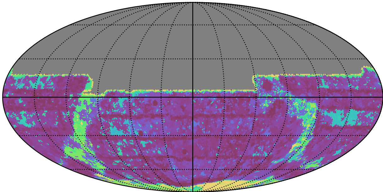
baseline_v3.2_10yrs All sky y band: Max Inter-Night Gap
