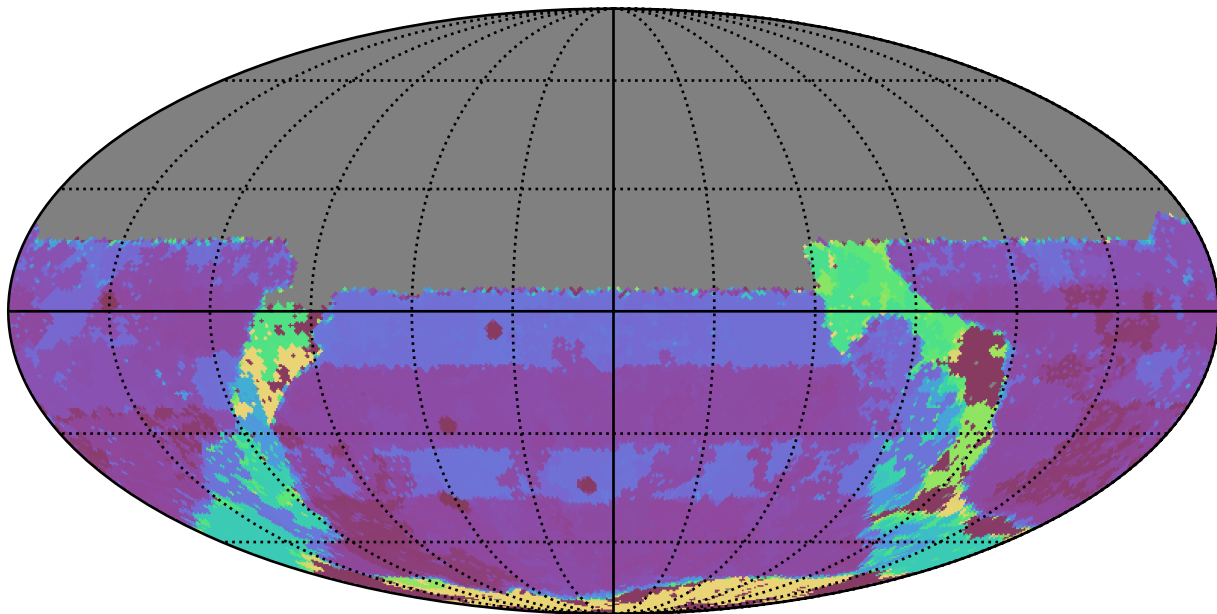
baseline_v3.2_10yrs All sky u band: Max Inter-Night Gap
