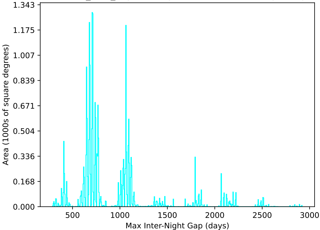
baseline_v3.2_10yrs All sky u band: Max Inter-Night Gap
