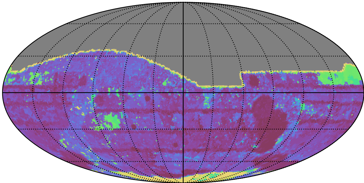
baseline_v3.2_10yrs All sky i band: Max Inter-Night Gap
