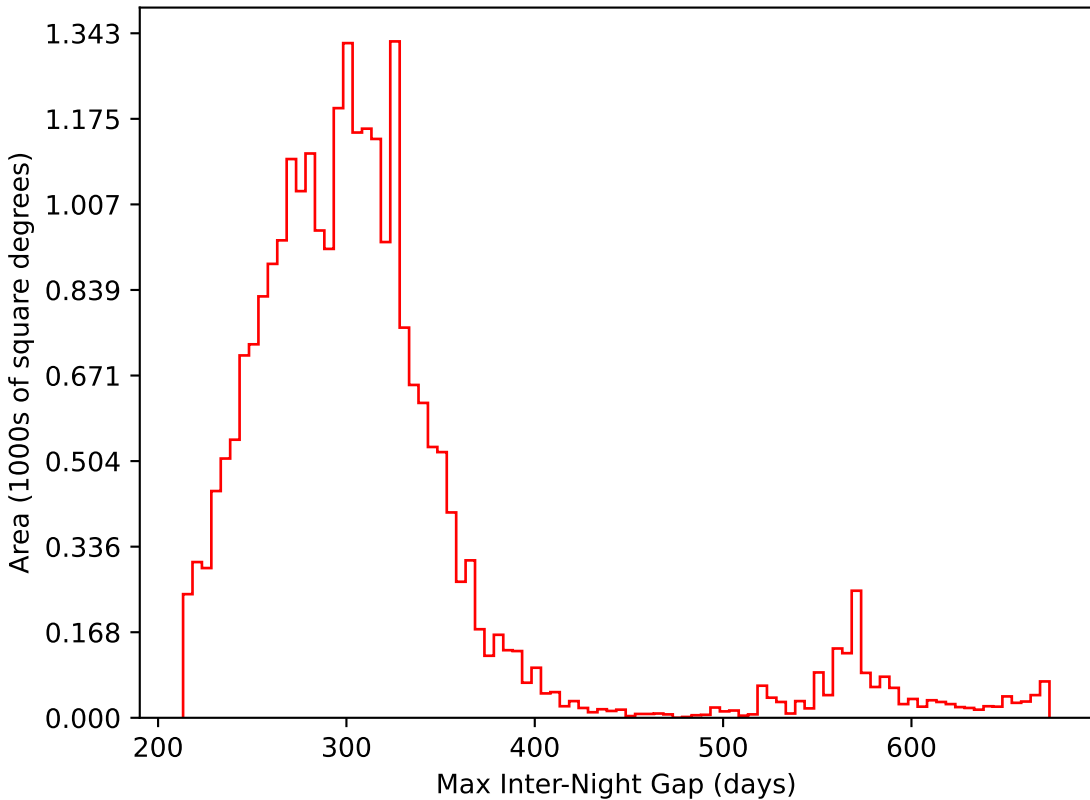
baseline_v3.2_10yrs All sky i band: Max Inter-Night Gap
