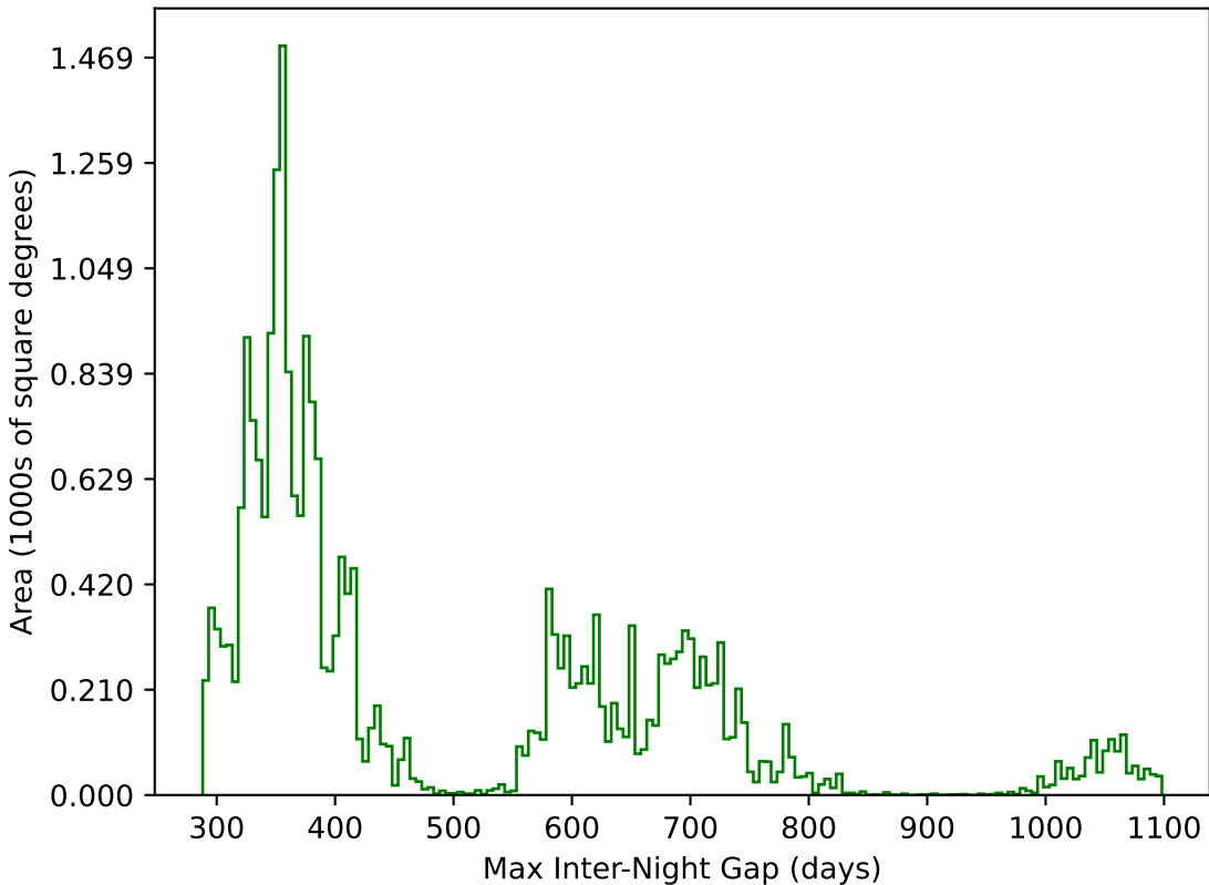
baseline_v3.2_10yrs All sky g band: Max Inter-Night Gap
