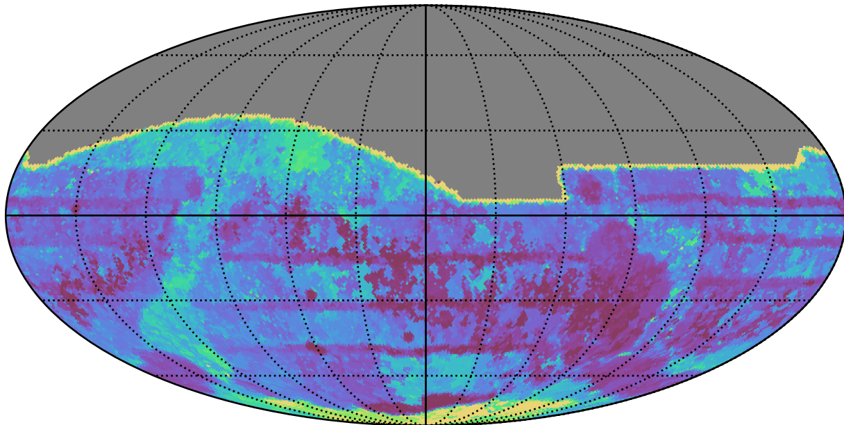
baseline_v3.2_10yrs All sky all bands: Max Inter-Night Gap
