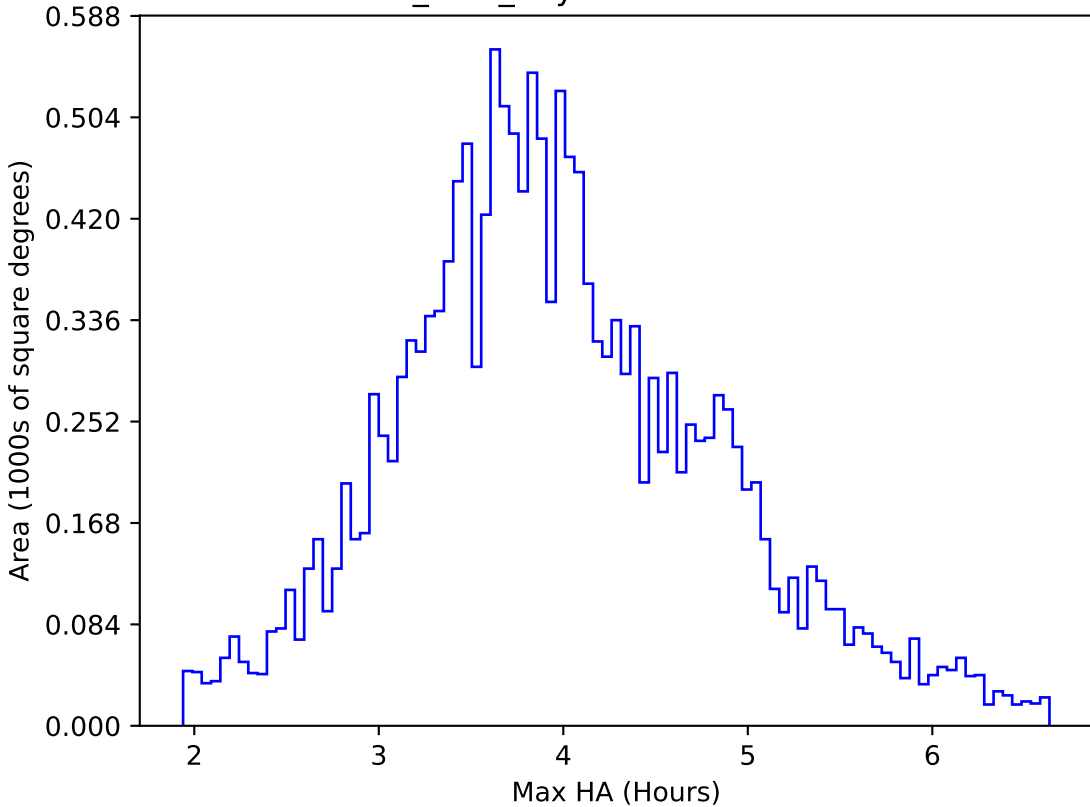
baseline_v3.2_10yrs WFD u band: Max HA
