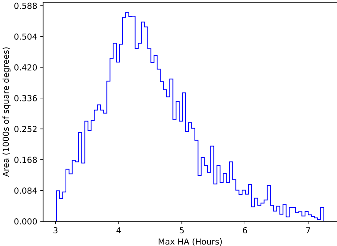
baseline_v3.2_10yrs WFD r band: Max HA
