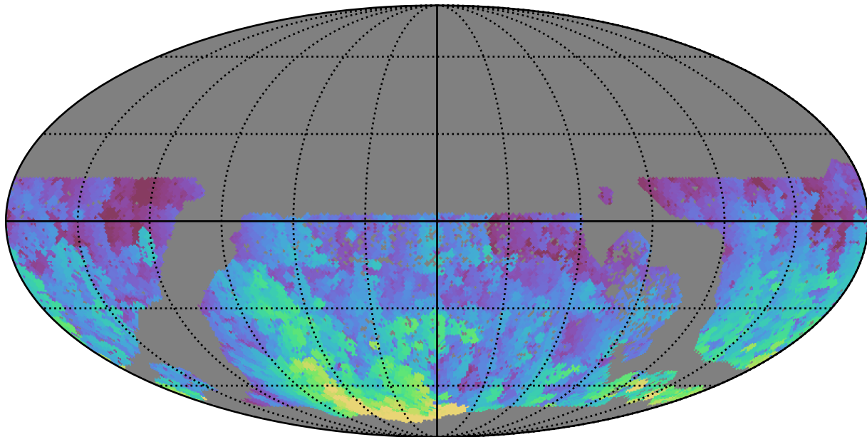
baseline_v3.2_10yrs WFD g band: Max HA
