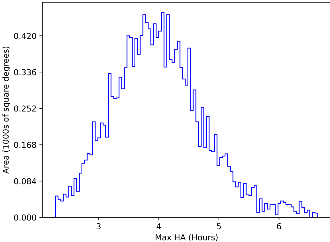
baseline_v3.2_10yrs WFD g band: Max HA
