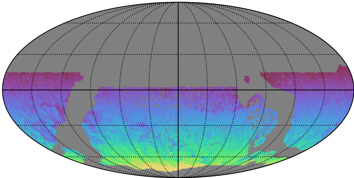
baseline_v3.2_10yrs WFD all bands: Max HA
