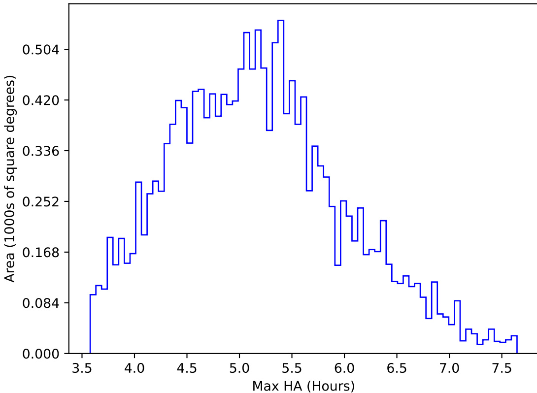
baseline_v3.2_10yrs WFD all bands: Max HA
