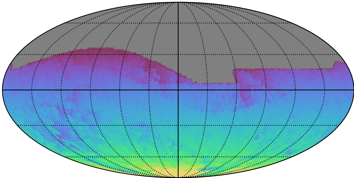
baseline_v3.2_10yrs All sky all bands: Max HA
