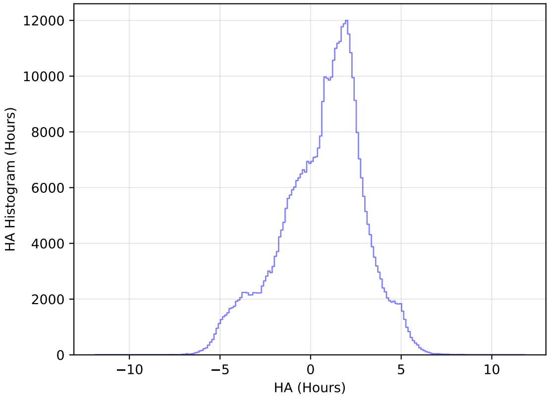
baseline_v3.2_10yrs WFD z band: HA Histogram
