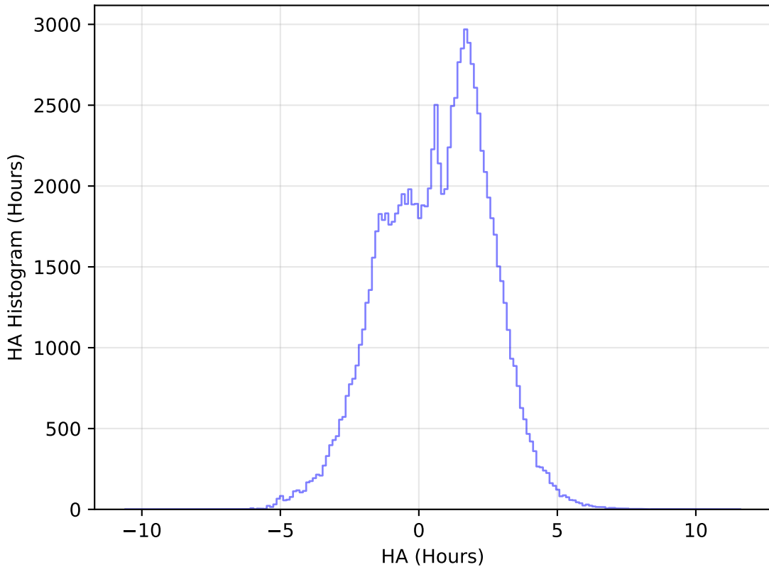
baseline_v3.2_10yrs WFD u band: HA Histogram
