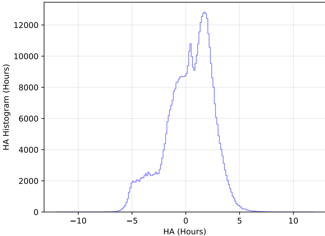
baseline_v3.2_10yrs WFD r band: HA Histogram
