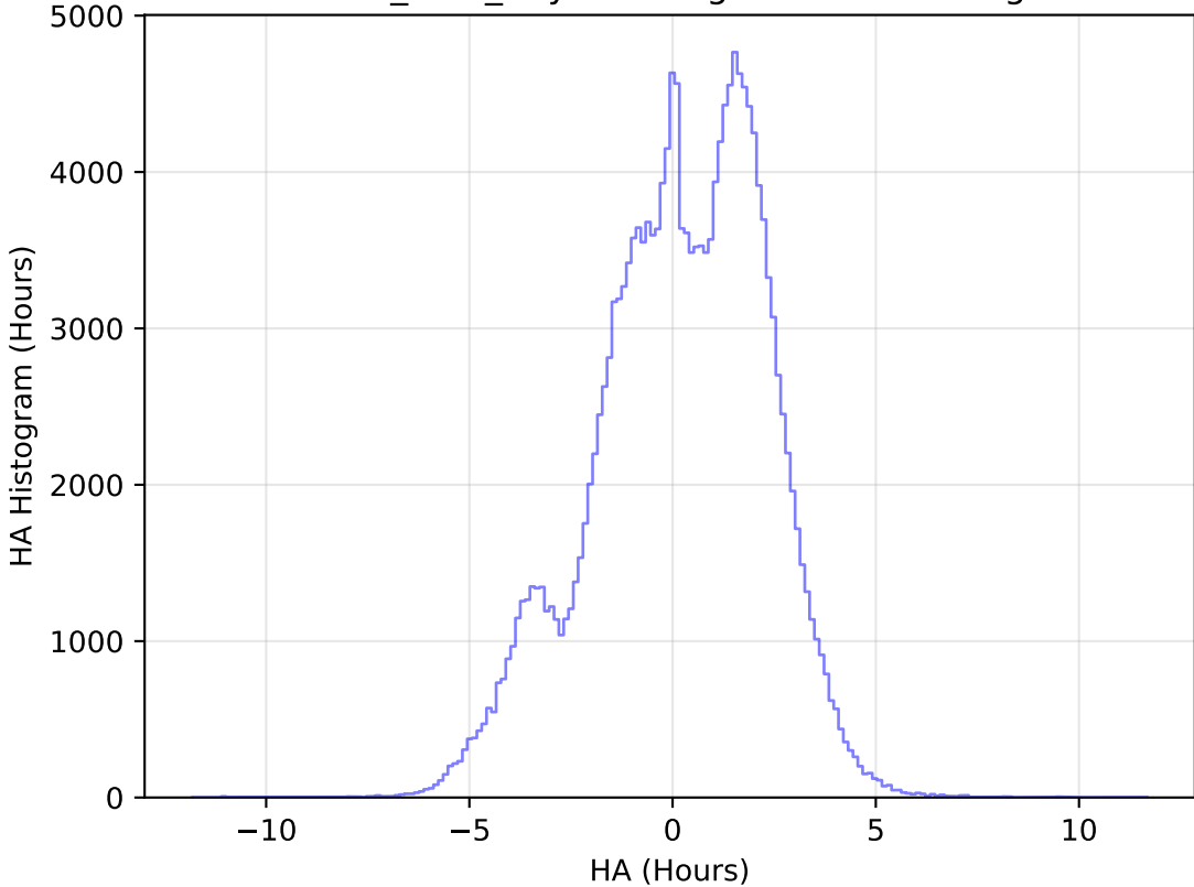
baseline_v3.2_10yrs WFD g band: HA Histogram
