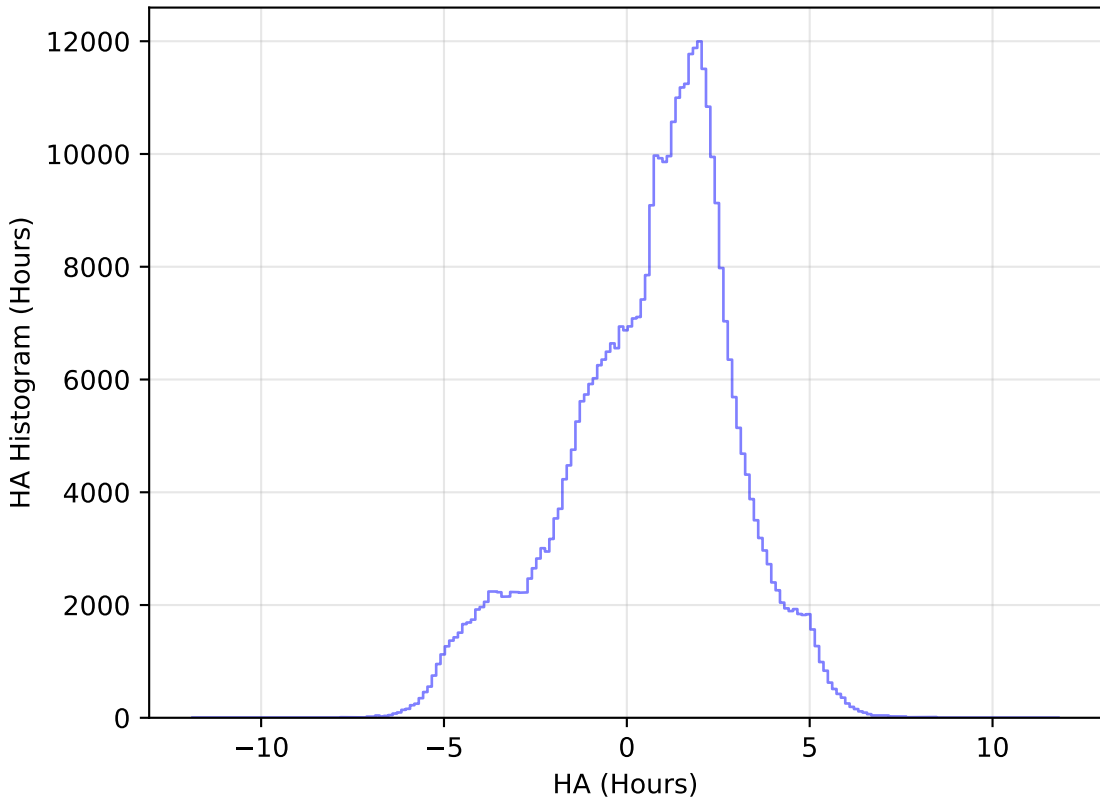
baseline_v3.2_10yrs All sky z band: HA Histogram
