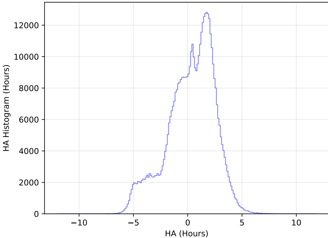
baseline_v3.2_10yrs All sky r band: HA Histogram
