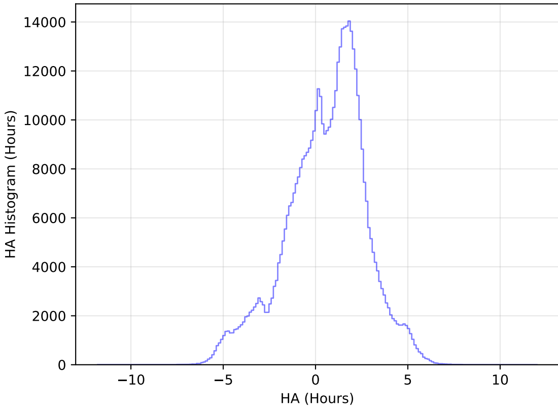
baseline_v3.2_10yrs All sky i band: HA Histogram
