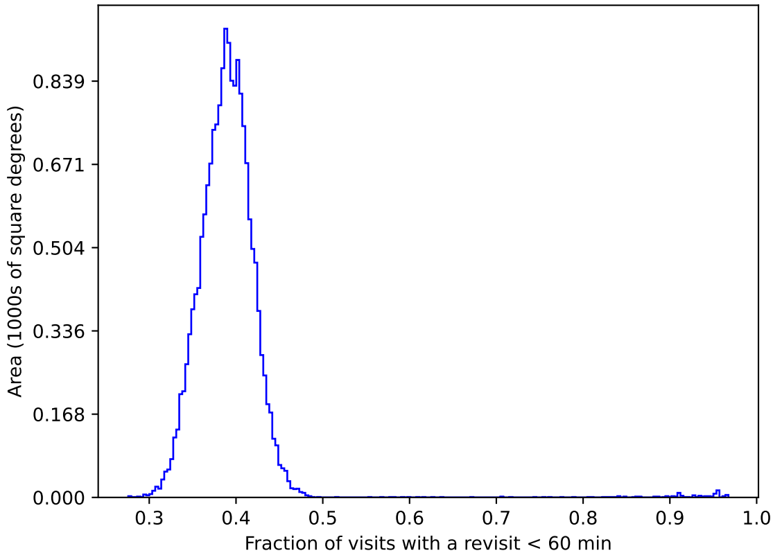
baseline_v3.2_10yrs gri WFD: Fraction of visits with a revisit < 60 min
