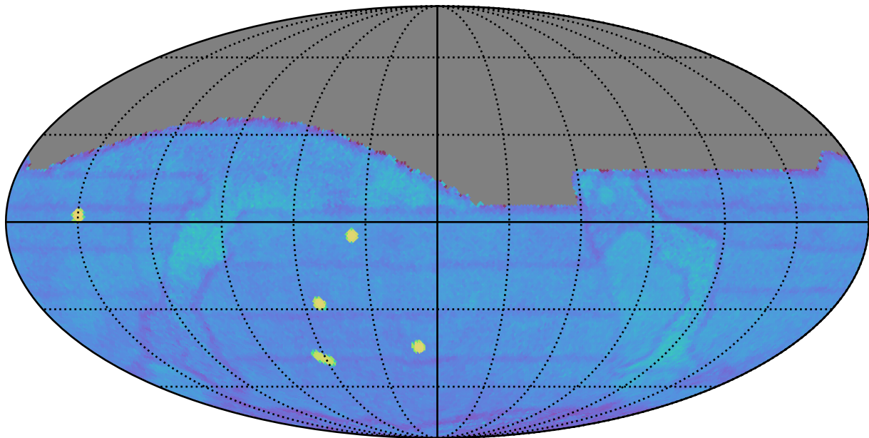
baseline_v3.2_10yrs gri All sky: Fraction of visits with a revisit < 60 min
