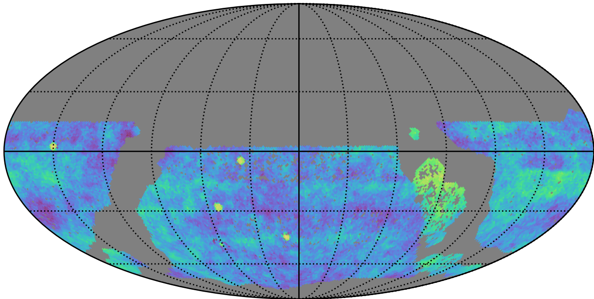
baseline_v3.2_10yrs gri WFD: Fraction of visits in pairs (20-90 min)
