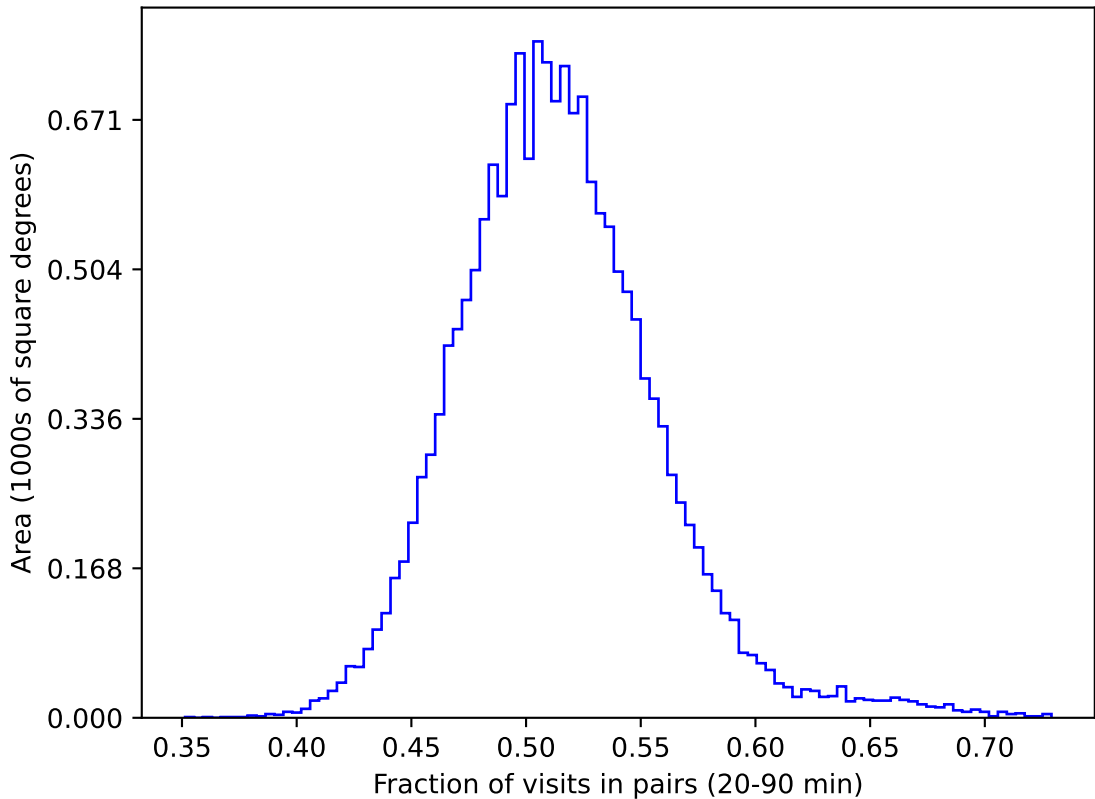
baseline_v3.2_10yrs gri WFD: Fraction of visits in pairs (20-90 min)
