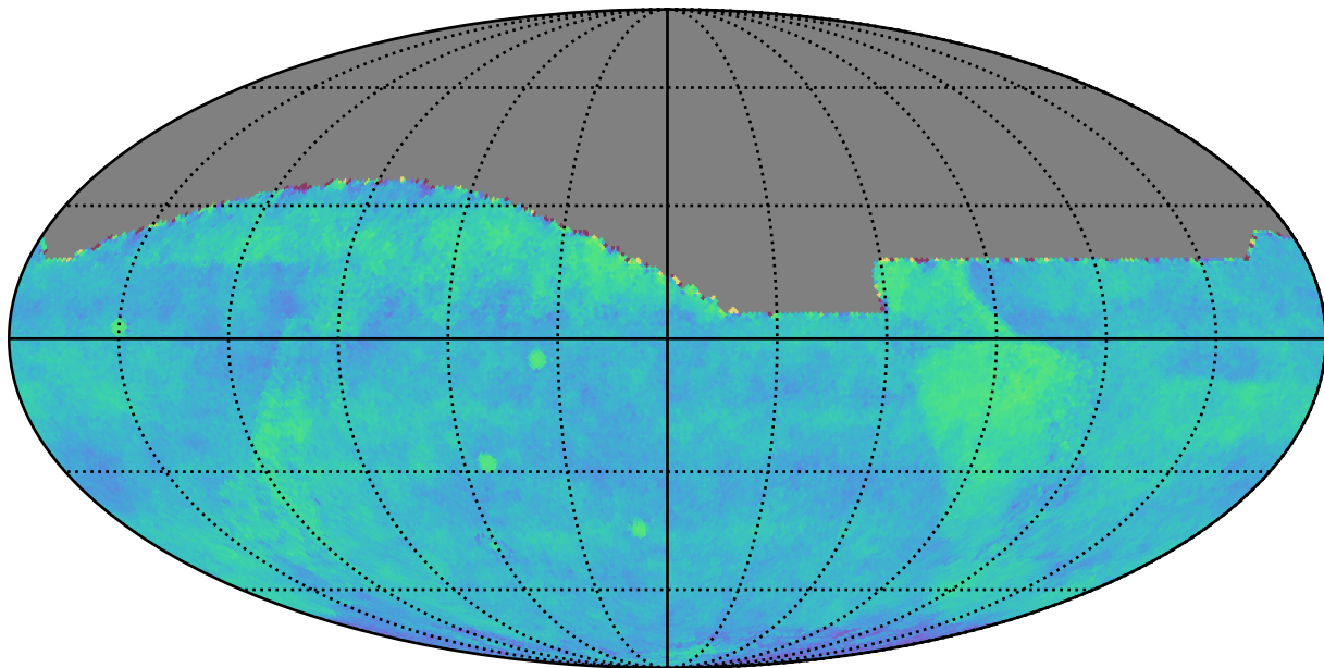
baseline_v3.2_10yrs gri All sky: Fraction of visits in pairs (20-90 min)
