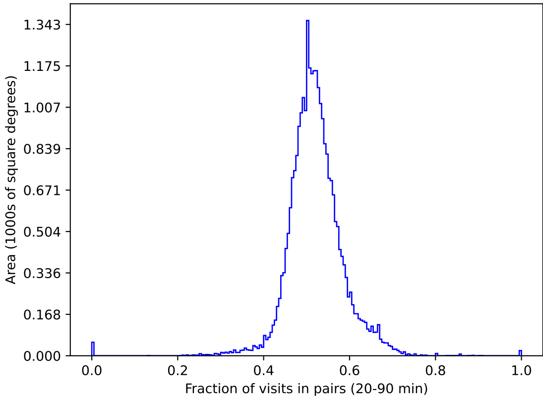
baseline_v3.2_10yrs gri All sky: Fraction of visits in pairs (20-90 min)
