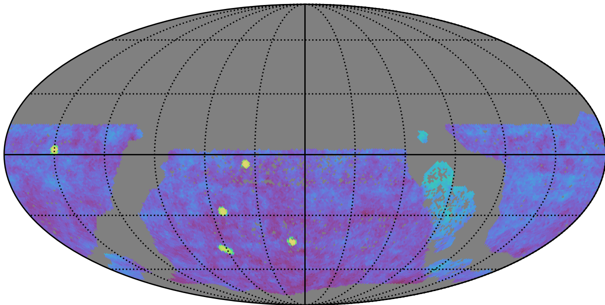
baseline_v3.2_10yrs gri WFD: Fraction of visits in pairs (10-60 min)
