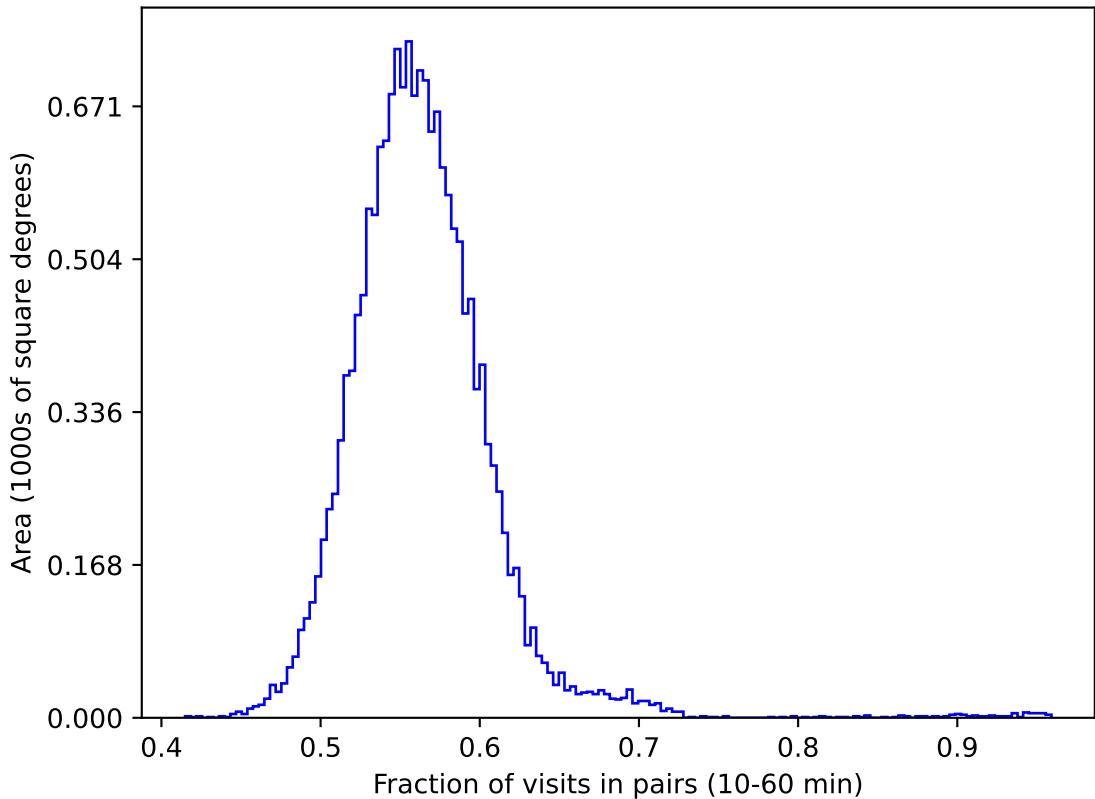
baseline_v3.2_10yrs gri WFD: Fraction of visits in pairs (10-60 min)
