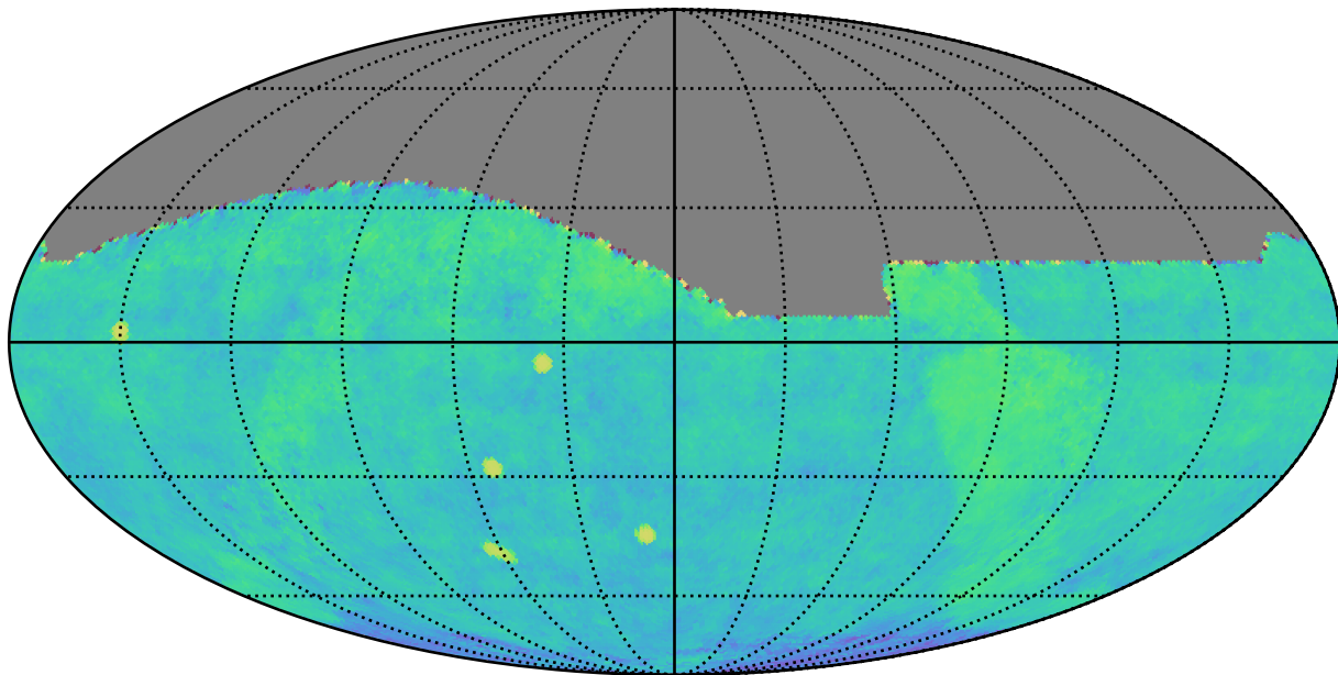
baseline_v3.2_10yrs gri All sky: Fraction of visits in pairs (10-60 min)
