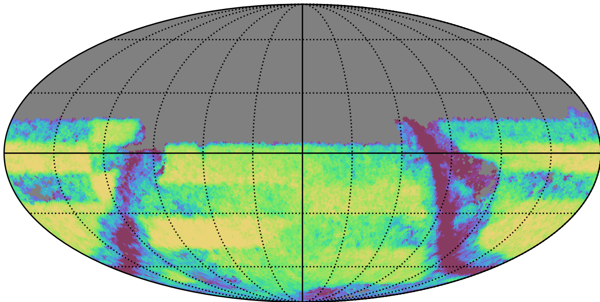
baseline_v3.2_10yrs Yr 3-4 y band: Exgal_CoaddM5
