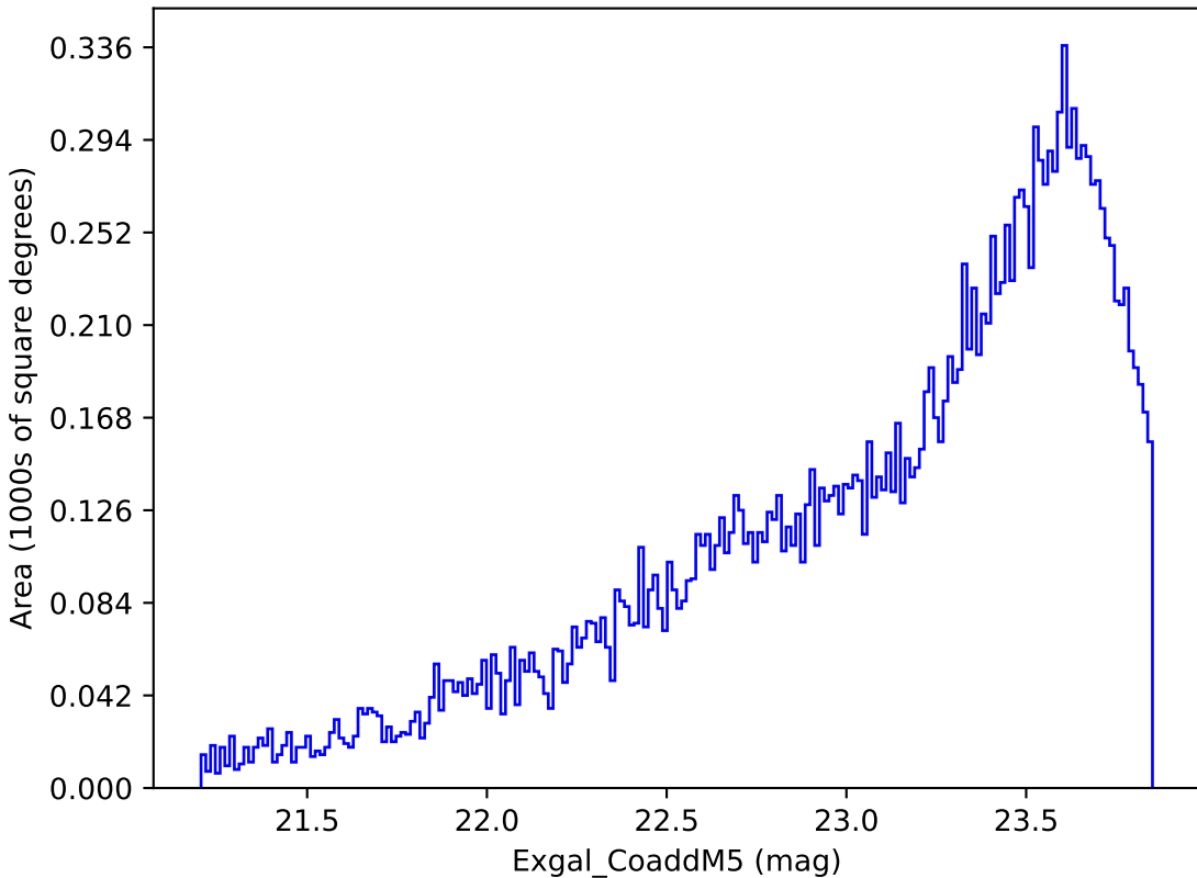
baseline_v3.2_10yrs Yr 3-4 y band: Exgal_CoaddM5
