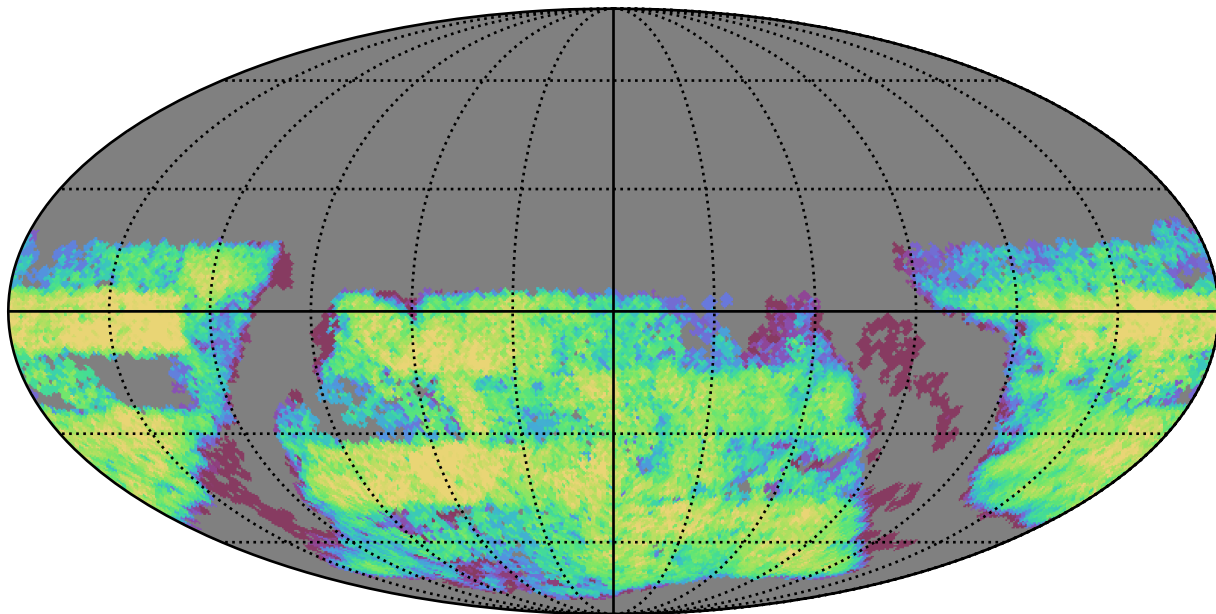
baseline_v3.2_10yrs Yr 3-4 u band: Exgal_CoaddM5
