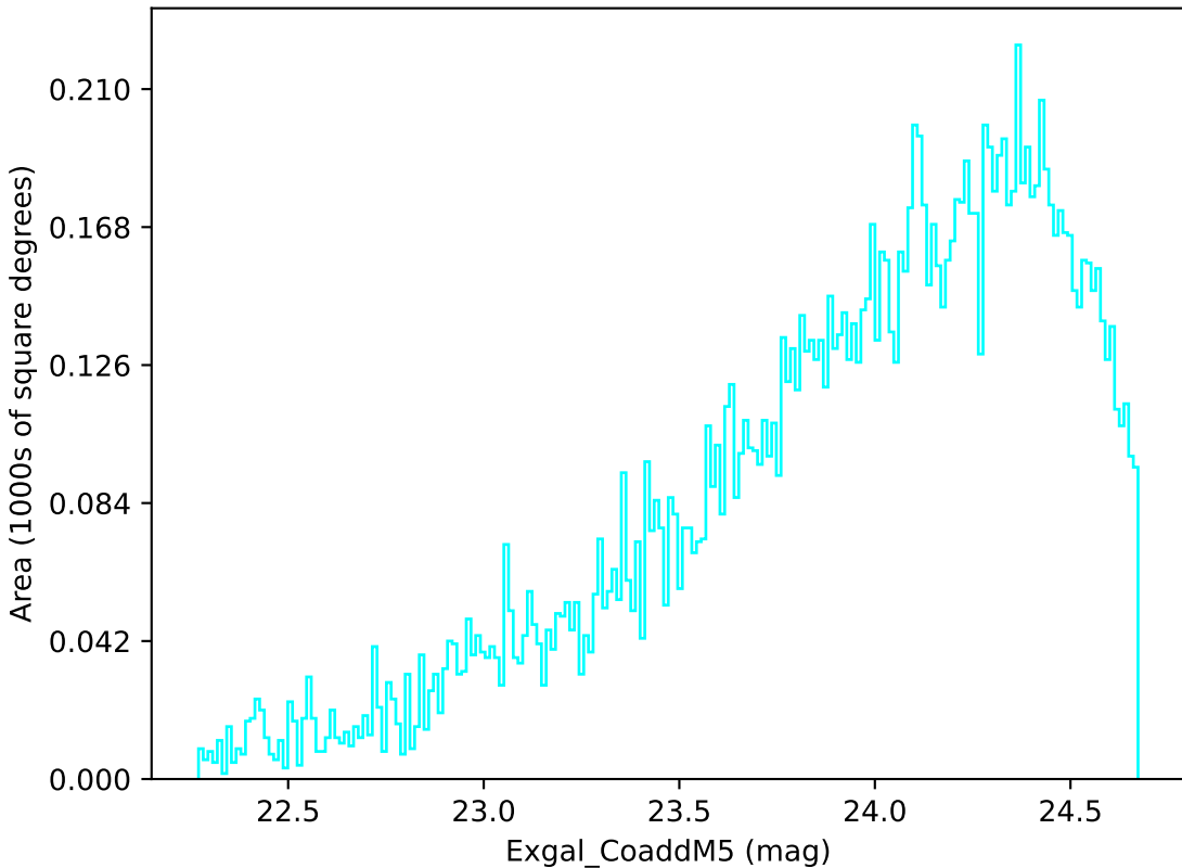
baseline_v3.2_10yrs Yr 3-4 u band: Exgal_CoaddM5
