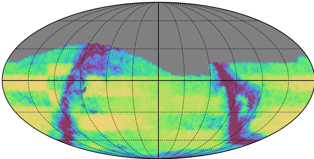
baseline_v3.2_10yrs Yr 3-4 r band: Exgal_CoaddM5
