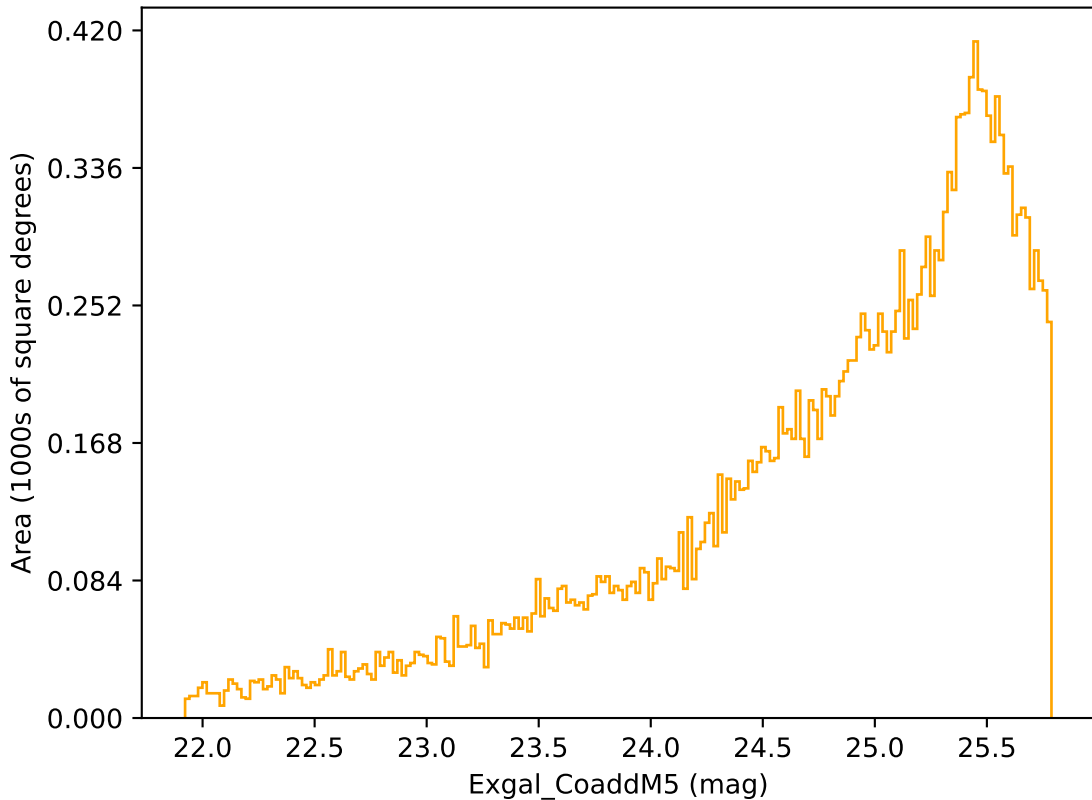
baseline_v3.2_10yrs Yr 3-4 r band: Exgal_CoaddM5
