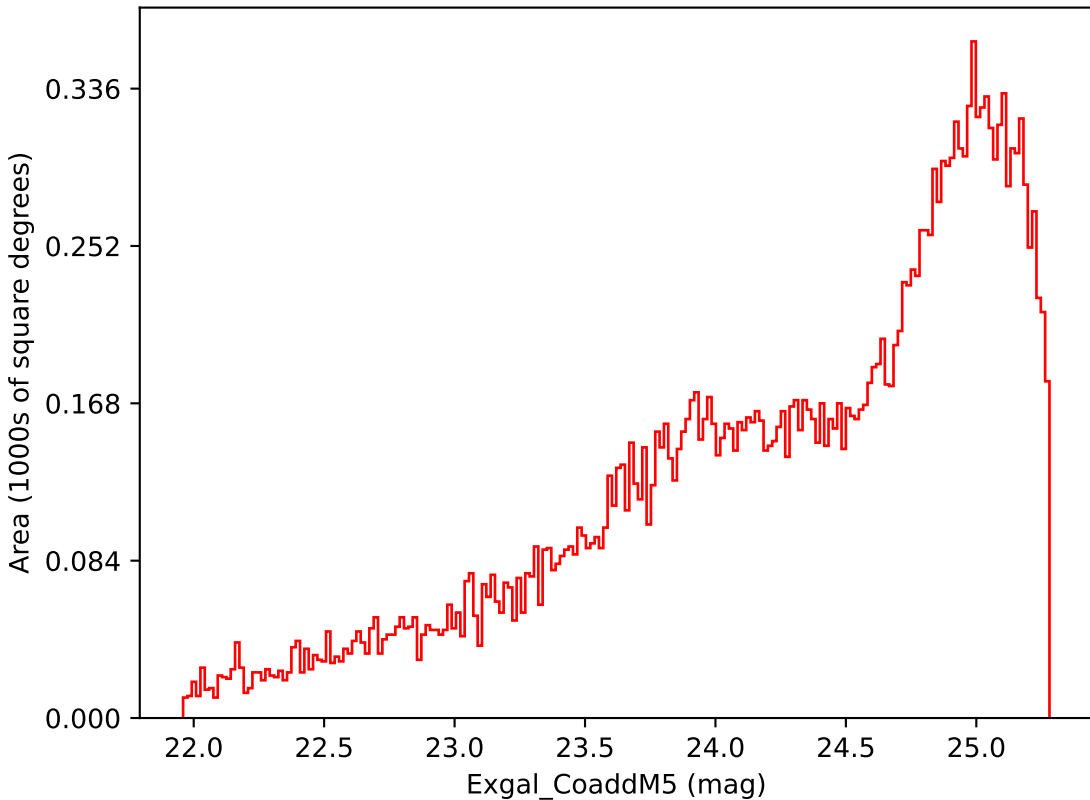
baseline_v3.2_10yrs Yr 3-4 i band: Exgal_CoaddM5
