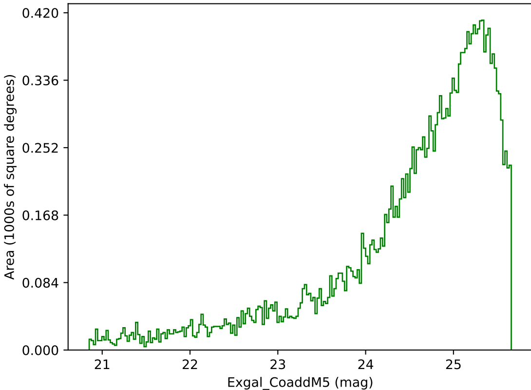
baseline_v3.2_10yrs Yr 3-4 g band: Exgal_CoaddM5
