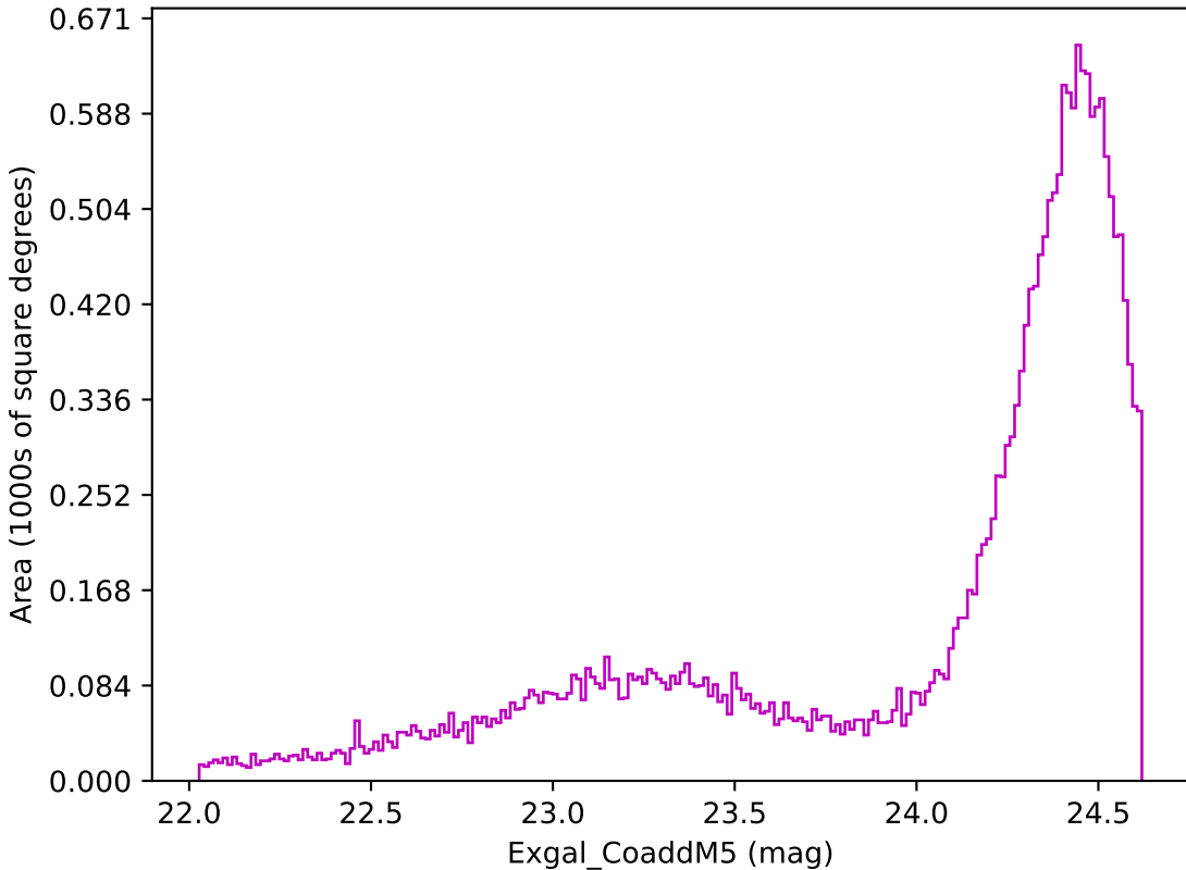
baseline_v3.2_10yrs Yr 1 z band: Exgal_CoaddM5
