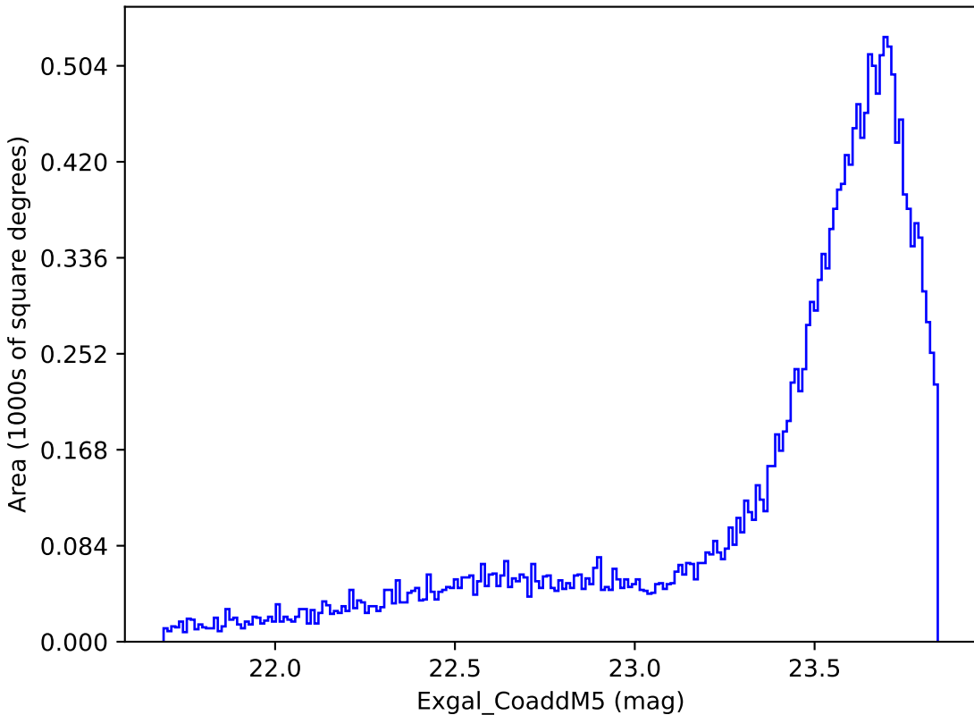
baseline_v3.2_10yrs Yr 1 y band: Exgal_CoaddM5
